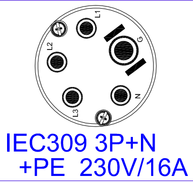
VIEW A
